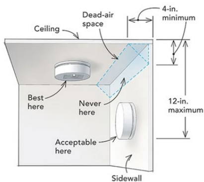
Where to install Smoke/Carbon Monoxide Alarms
